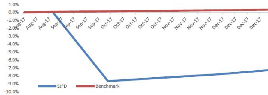
Inception Performance
